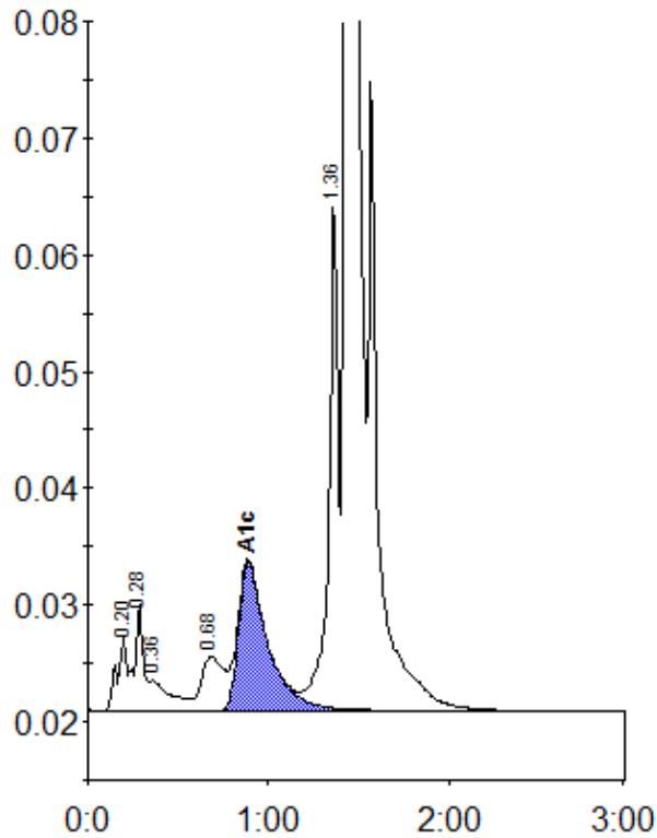
Peak table - ID: 10213449
